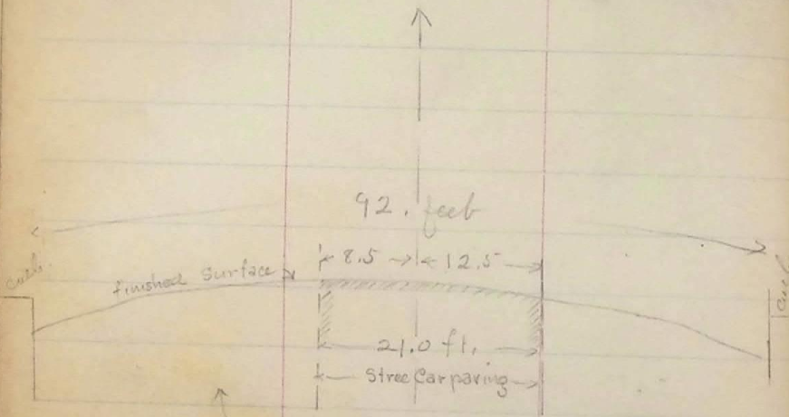
Cross-section to show the portion of street to be paved at the expense of the Street Railway Co, bet 22 nd and 23 rd St.
